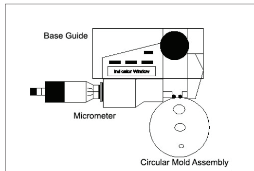
Mold Assembly, Micrometer & Base Guide
